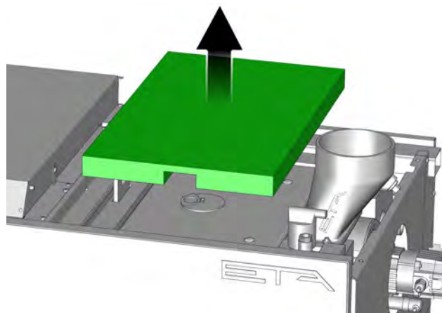
Fig. 2-16: Isolation
